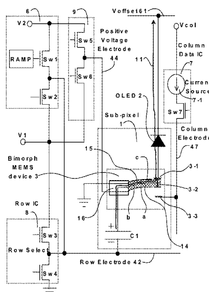
BIMORPH MEMS DEVICE POSITIONED LIGHT EMISSION
